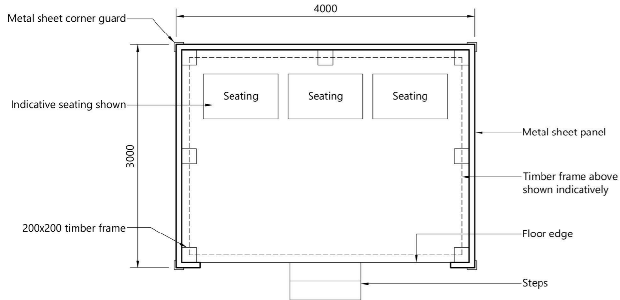
Floor Plan
